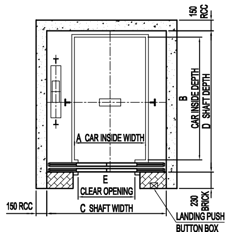
Cross Sectional Plan Of Elevator Shaft (Center Opening Door)
