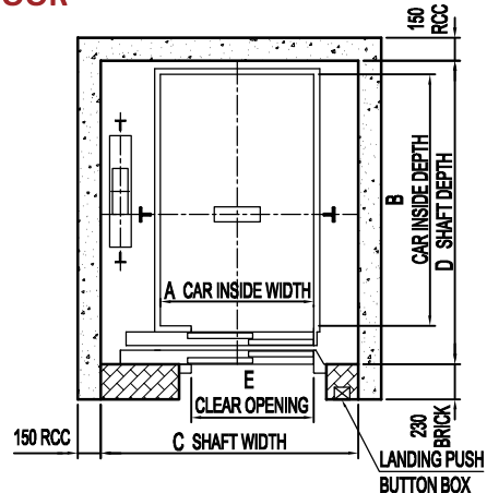
Cross Sectional Plan Of Elevator Shaft (Telescopic Door)
