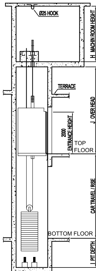
Sectional Elevation Of Elevator Shaft
